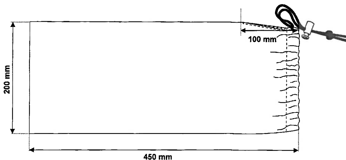
Figure 5 - Dimensions of storage bag
