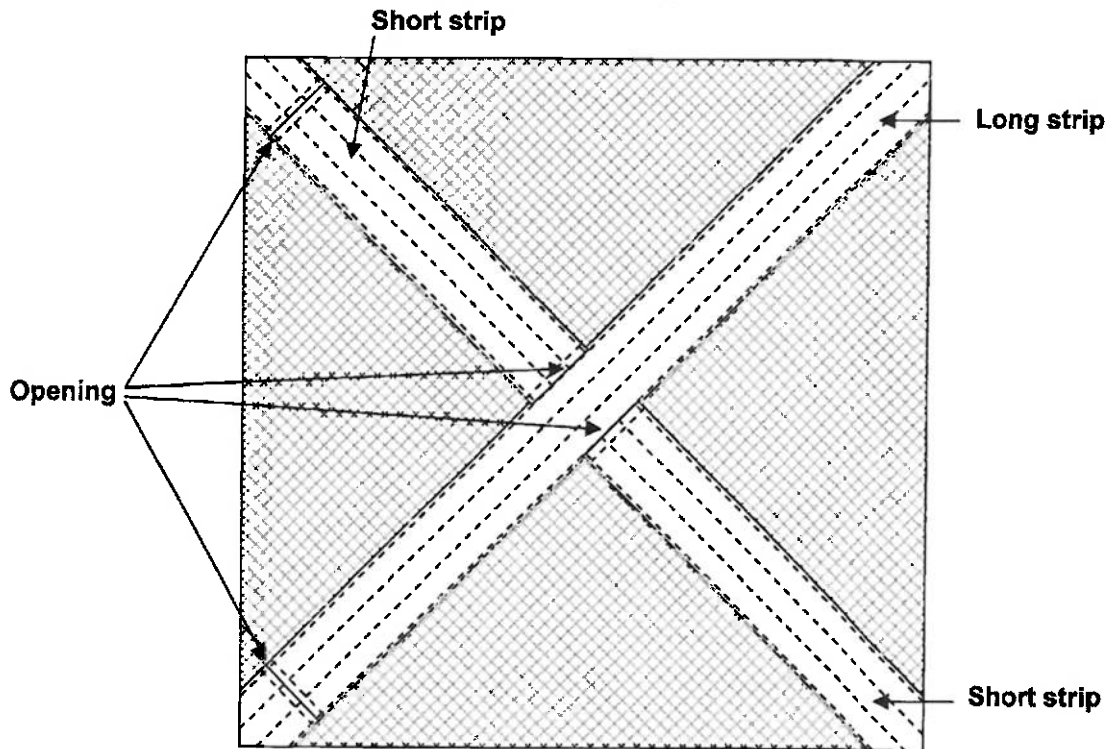
Figure 7 – Top panel
