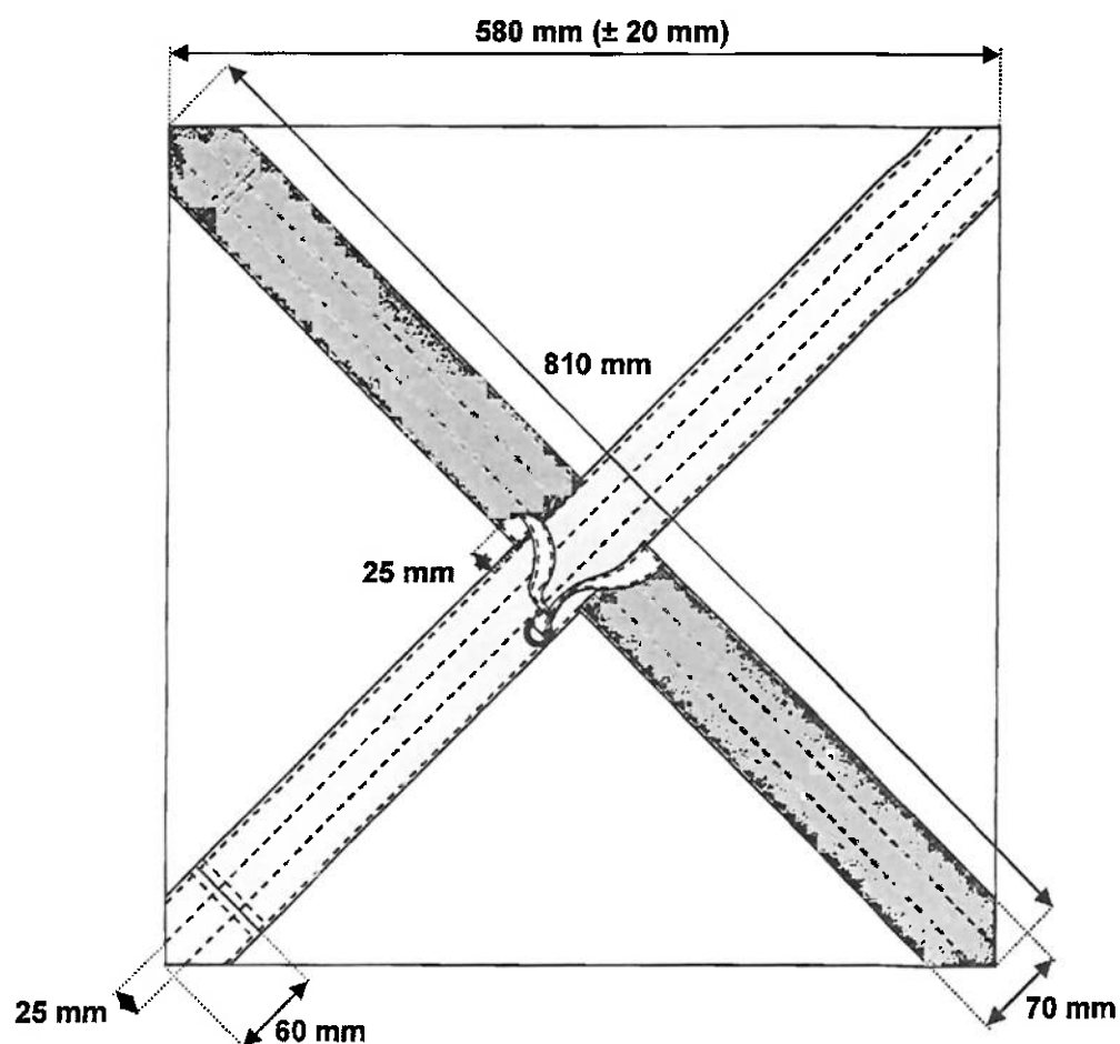
Figure 4 - Dimensions of top panel and attached components
