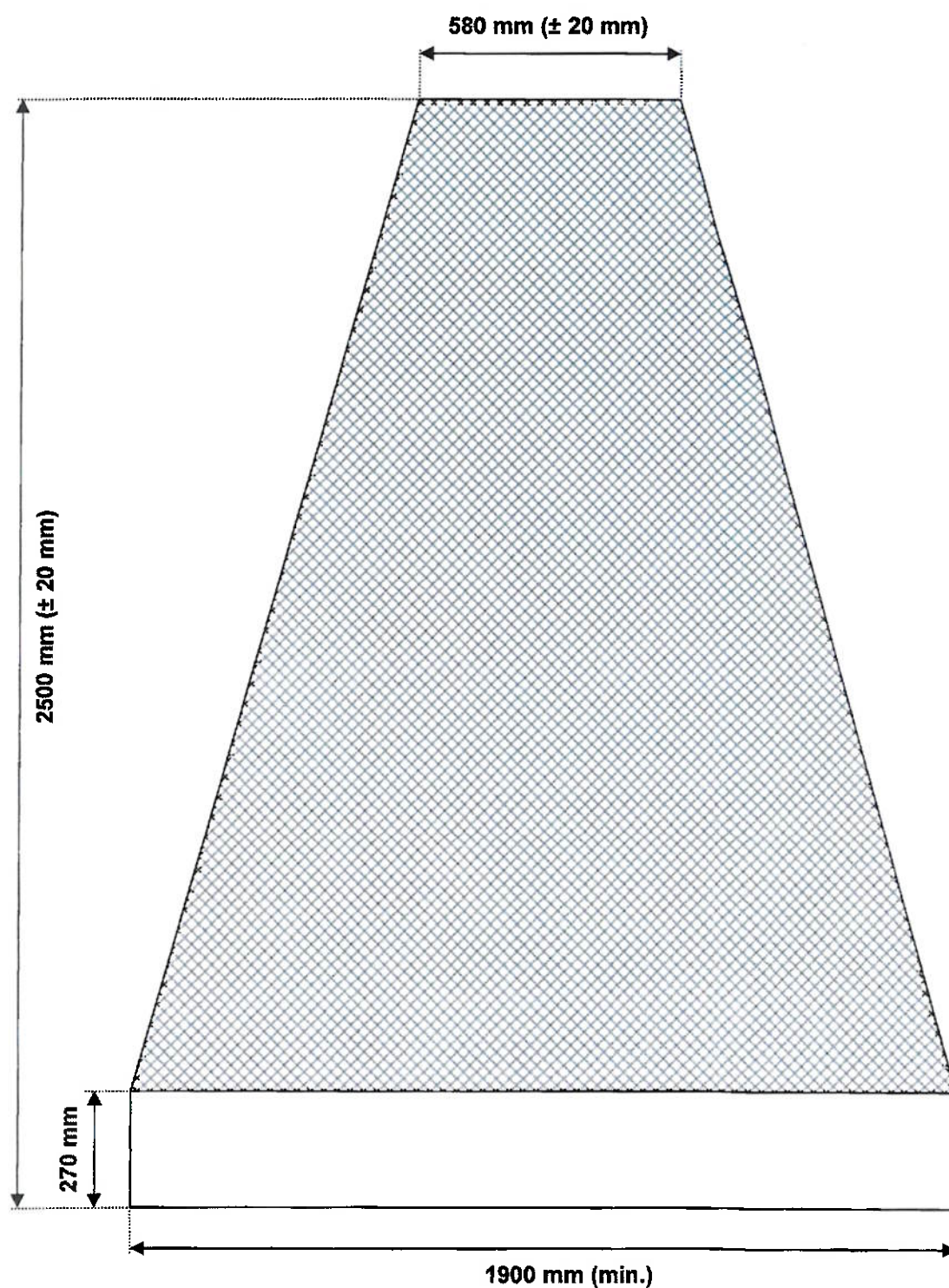
Figure 3 - Dimensions of each side panel of the Mosquito Net, Cot Type
