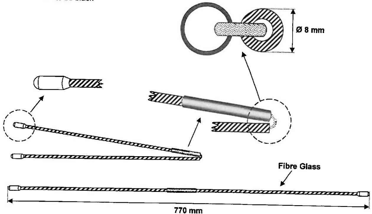
Figure 2 - Spreaders
