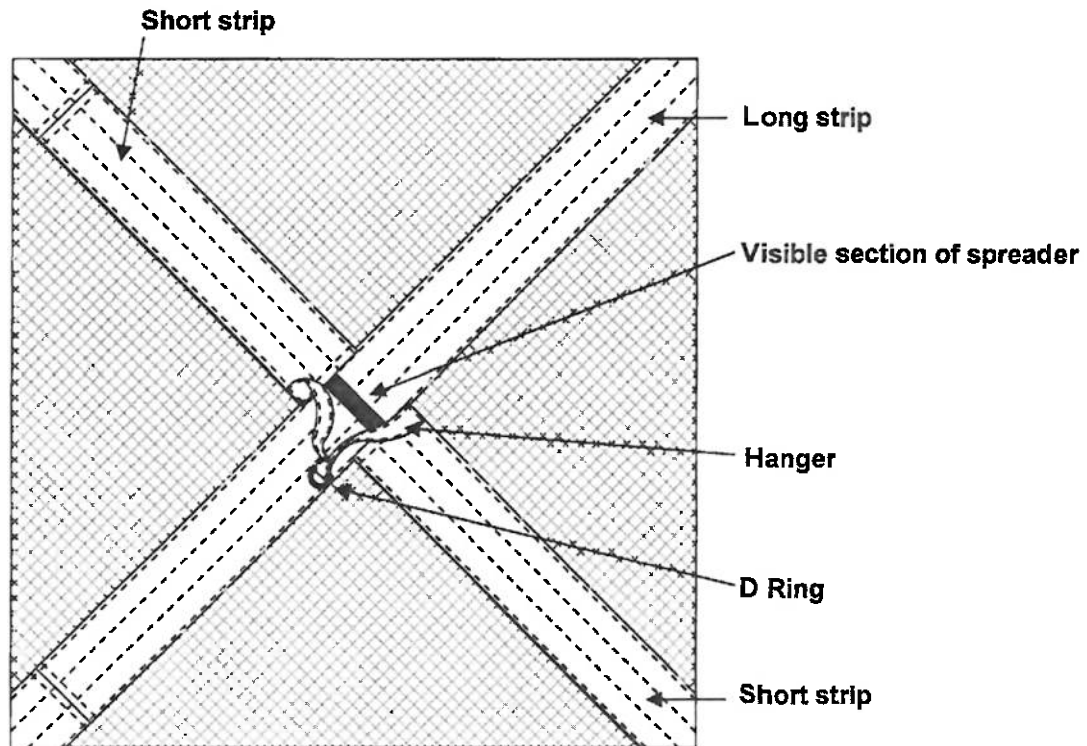
Figure 8 - Hanger attachment
