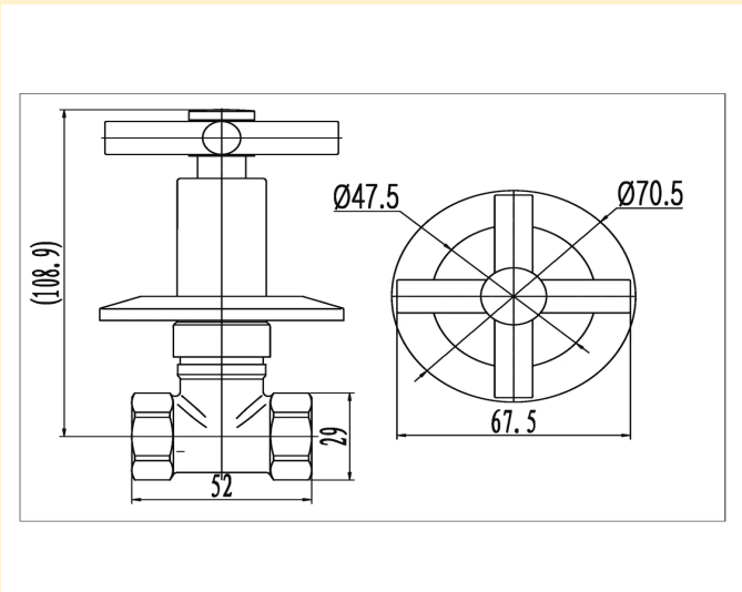
Stainless Steel Undertile Bath or Shower Stop Tap - 15mm
