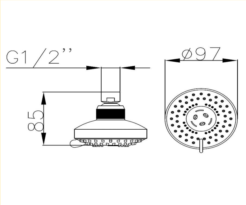
ITD Chrome 3-Function Round Shower Head (Equally Approved).
