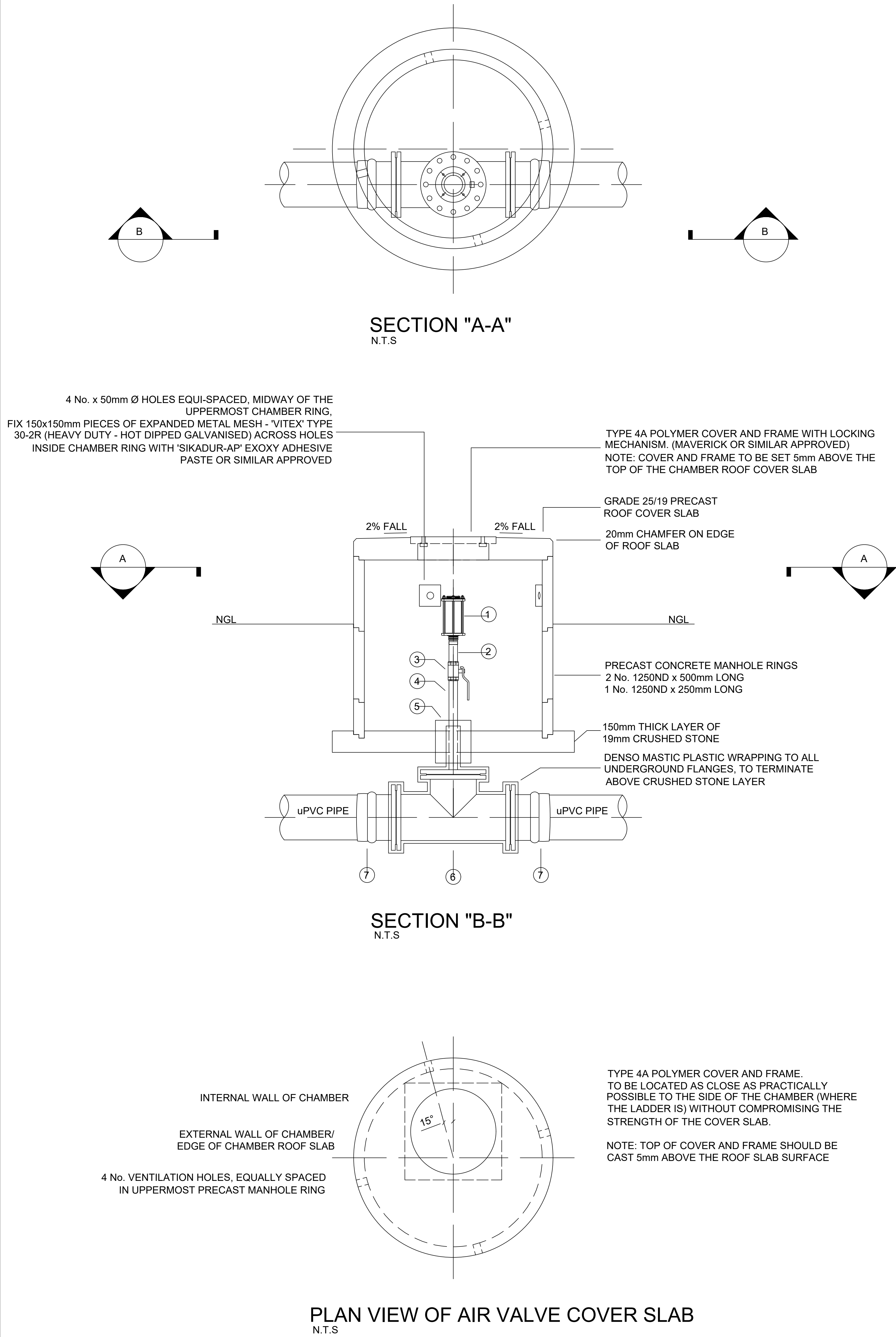
TYPICAL DETAILS FOR AIR VALVE INSTALLATION
