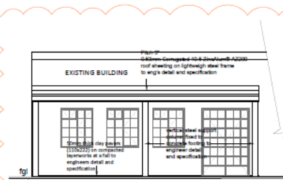
ELEVATION C SCALE 1:50
