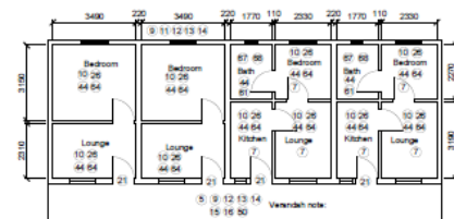
FLOOR PLAN - Nurses home scale 1:100
